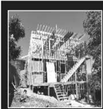
NEW Construction
